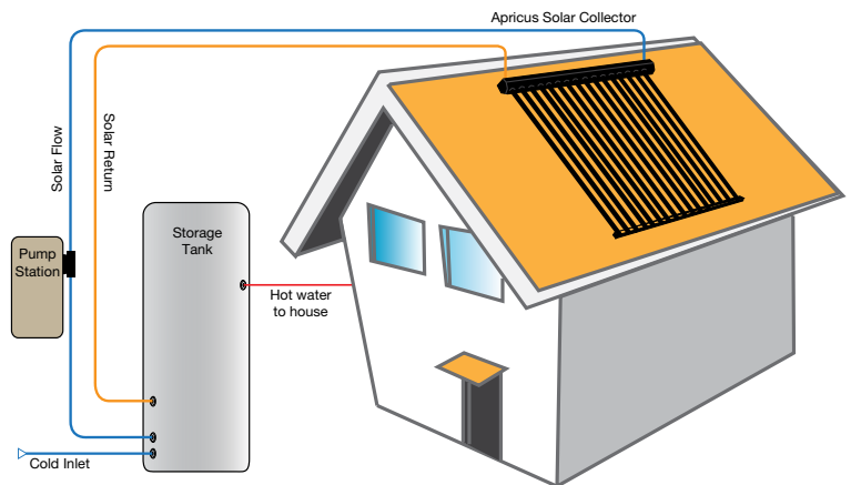
Note: Diagram not to scale - basic system overview not installation guide.
